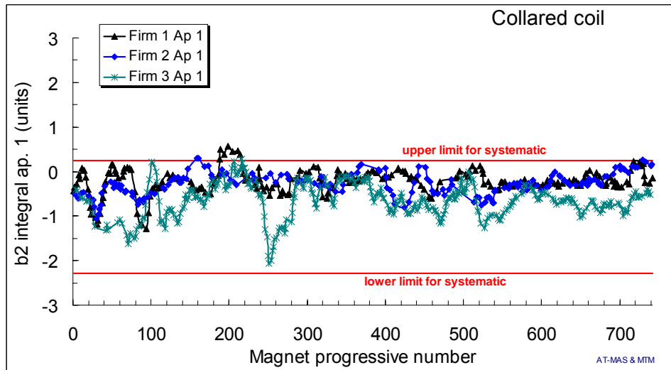
Fig. 17: Average b2 in straight part of the collared coils (aperture 1), separated per Firm (each dot is average of 5 consecutive magnets of the same Firm), and beam dynamics targets for the systematic (red lines) based on correlations with 134 cryodipoles.
