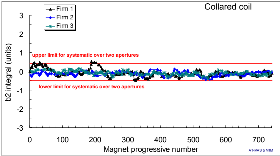
Fig. 19: Average b_2 in straight part of the collared coils (average of the apertures), separated per Firm (each dot is average of 5 consecutive magnets of the same Firm), and beam dynamics targets for the systematic (red lines) based on correlations with 134 cryodipoles.
