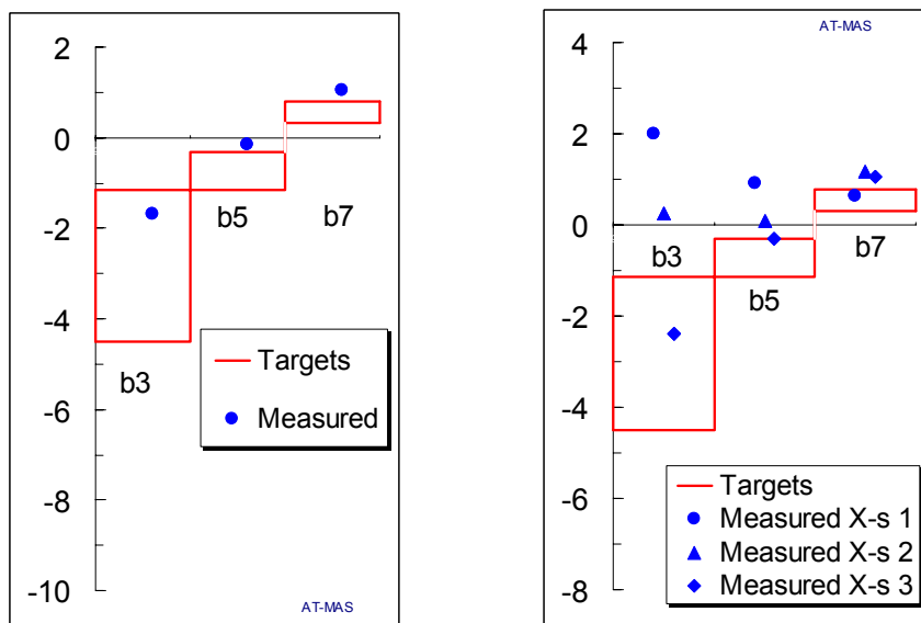
Fig. 4: Best estimate for systematic odd normal multipoles (markers) versus beam dynamics limits (red line). Raw data (left) and data separated according to different cross-sections (right).
