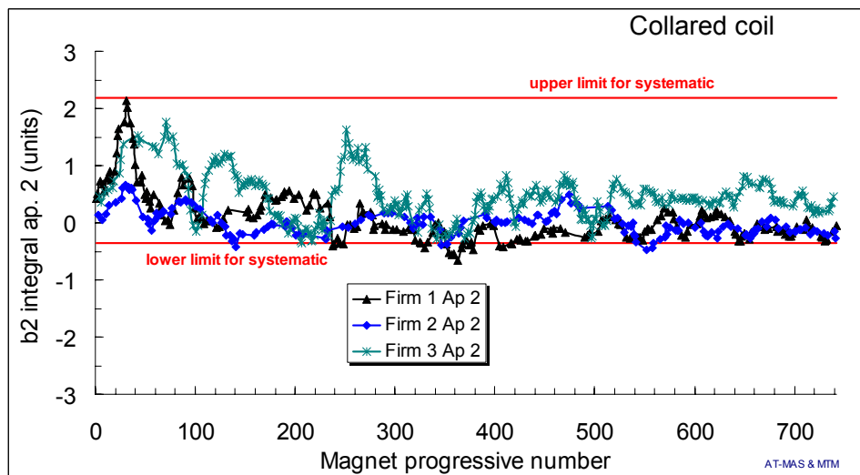
Fig. 18: Average b2 in straight part of the collared coils (aperture 2), separated per Firm (each dot is average of 5 consecutive magnets of the same Firm), and beam dynamics targets for the systematic (red lines) based on correlations with 134 cryodipoles.
