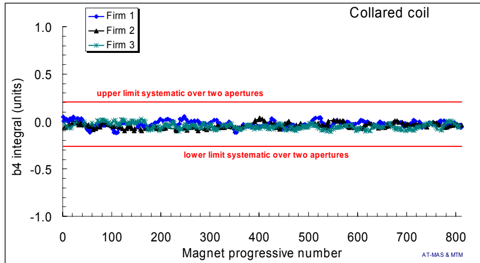
Fig. 22: Average b4 in straight part of the collared coils (average of the apertures), separated per Firm (each dot is average of 5 consecutive magnets of the same Firm), and beam dynamics targets for the systematic (red lines) based on correlations with 144 cryodipoles.
