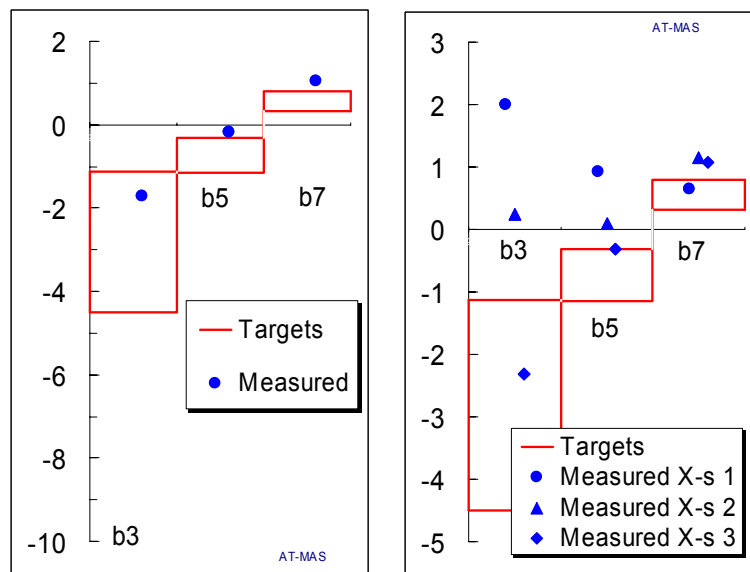
Fig. 4: Best estimate for systematic odd normal multipoles (markers) versus beam dynamics limits (solid red line). Raw data (left) and data separated according to different cross-sections (right).
