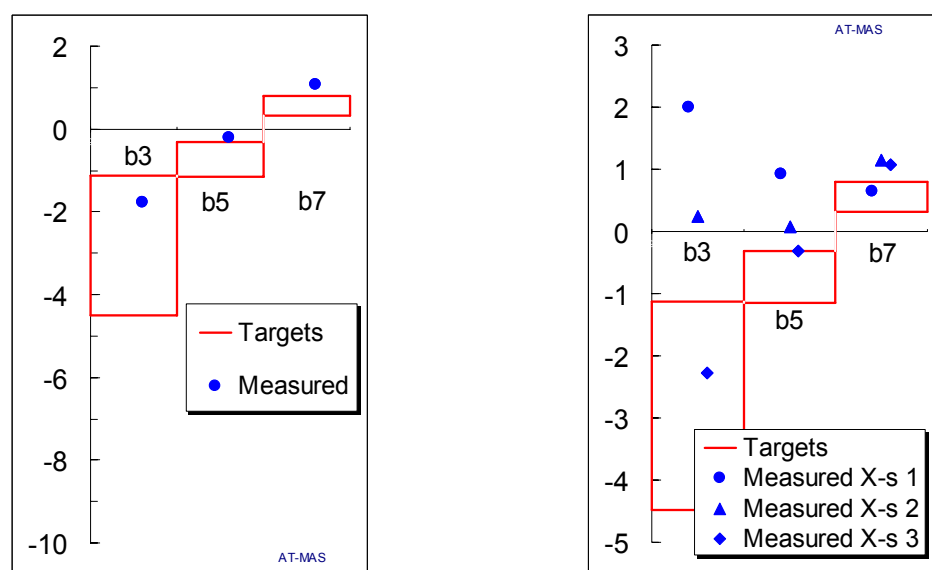
Fig. 4: Best estimate for systematic odd normal multipoles (markers) versus beam dynamics limits (solid red line). Raw data (left) and data separated according to different cross-sections (right).
