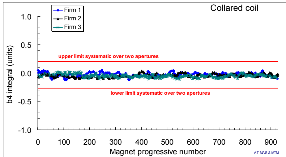
Fig. 22: Average b4 in straight part of the collared coils (average of the apertures), separated per Firm (each dot is the average of 5 consecutive magnets of the same Firm), and beam dynamics targets for the systematic (red lines) based on correlations with 156 cryodipoles.
