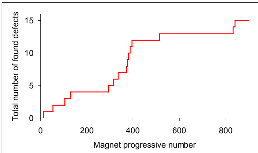
Fig. 32: Total number of defects found with room temperature magnetic measurements versus magnet progressive number.
