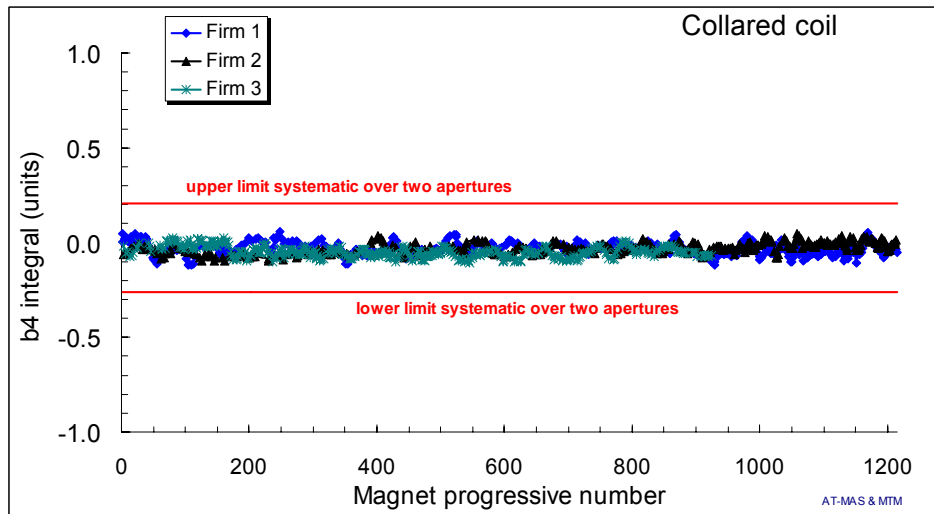
Fig. 22: Integral b_4 in the collared coils (average of the apertures), separated per Firm (each dot is the average of 5 consecutive magnets of the same Firm), and beam dynamics targets for the systematic (red lines) based on correlations with 183 cryodipoles.
