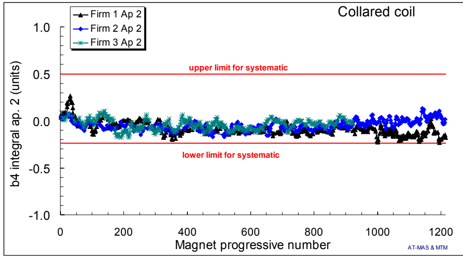
Fig. 21: Integral b_4 in the collared coils (aperture 2), separated per Firm (each dot is the average of 5 consecutive magnets of the same Firm), and beam dynamics targets for the systematic (red lines) based on correlations with 183 cryodipoles.
