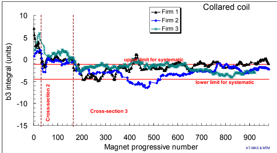
Fig. 13: Average b_3 in straight part of the collared coils, separated per Firm (each dot is the average of 5 consecutive magnets of the same Firm), and beam dynamics targets for the systematic (red lines) based on correlations with 163.5 cryodipoles.
