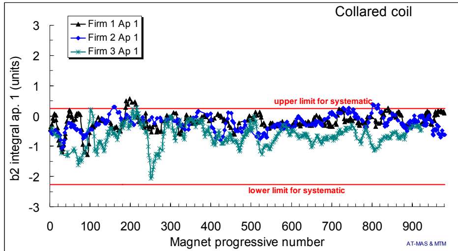
Fig. 17: Average b_2 in straight part of the collared coils (aperture 1), separated per Firm (each dot is the average of 5 consecutive magnets of the same Firm), and beam dynamics targets for the systematic (red lines) based on correlations with 163.5 cryodipoles.
