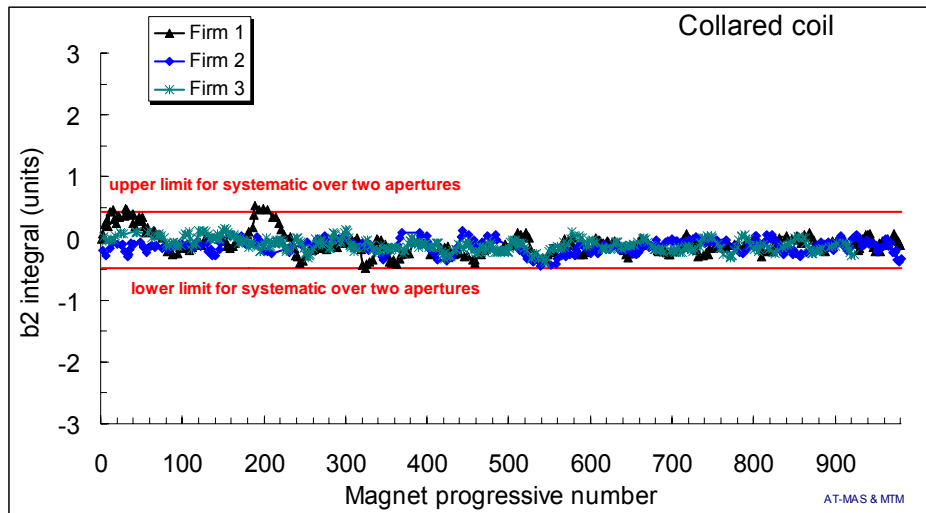
Fig. 19: Average b_2 in straight part of the collared coils (average of both apertures), separated per Firm (each dot is the average of 5 consecutive magnets of the same Firm), and beam dynamics targets for the systematic (red lines) based on correlations with 163.5 cryodipoles.
