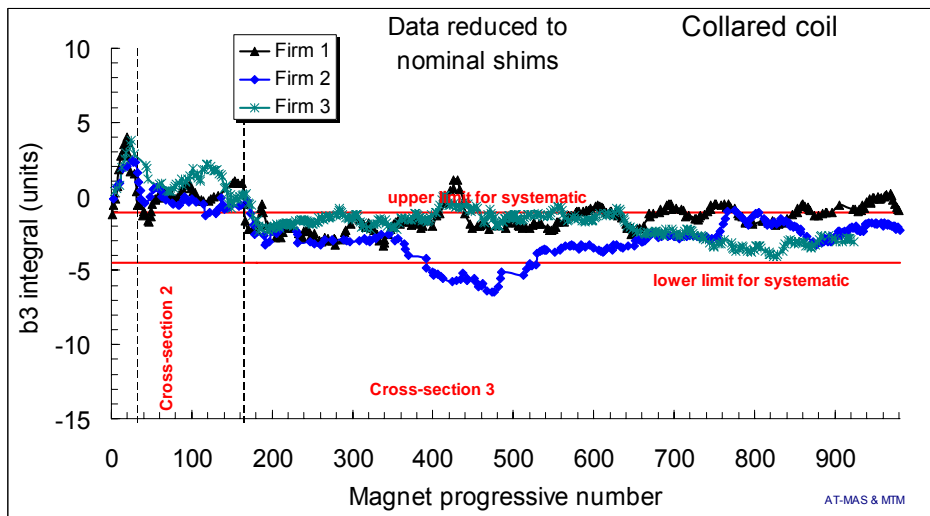
Fig. 14: Average b_3 in straight part of the collared coils, separated per Firm (each dot is the average of 5 consecutive magnets of the same Firm), and beam dynamics targets for the systematic (red lines) based on correlations with 163.5 cryodipoles. Data normalised to nominal shims 3 .
