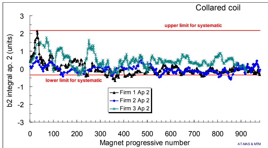
Fig. 18: Average b_2 in straight part of the collared coils (aperture 2), separated per Firm (each dot is the average of 5 consecutive magnets of the same Firm), and beam dynamics targets for the systematic (red lines) based on correlations with 163.5 cryodipoles.
