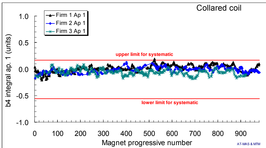
Fig. 20: Average b_4 in straight part of the collared coils (aperture 1), separated per Firm (each dot is the average of 5 consecutive magnets of the same Firm), and beam dynamics targets for the systematic (red lines) based on correlations with 163.5 cryodipoles.
