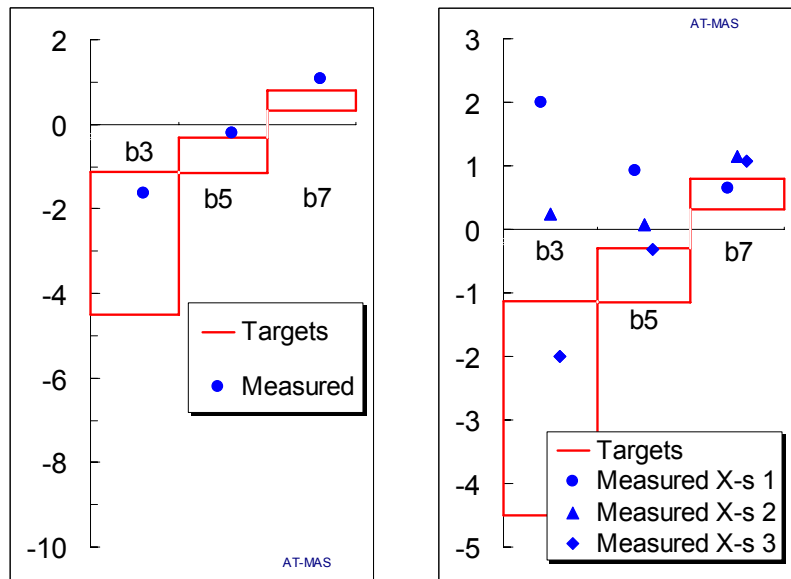
Fig. 4: Best estimate for systematic odd normal multipoles (markers) versus beam dynamics limits (solid red line). Raw data (left) and data separated according to different cross-sections (right).
