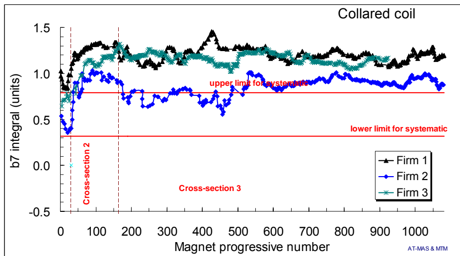
Fig. 16: Average b_7 in straight part of the collared coils, separated per Firm (each dot is the average of 5 consecutive magnets of the same Firm), and beam dynamics targets for the systematic (red lines) based on correlations with 176 cryodipoles.
