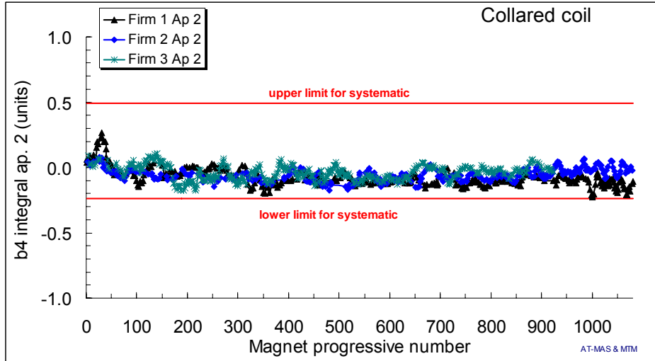
Fig. 21: Average b_4 in straight part of the collared coils (aperture 2), separated per Firm (each dot is the average of 5 consecutive magnets of the same Firm), and beam dynamics targets for the systematic (red lines) based on correlations with 176 cryodipoles.
