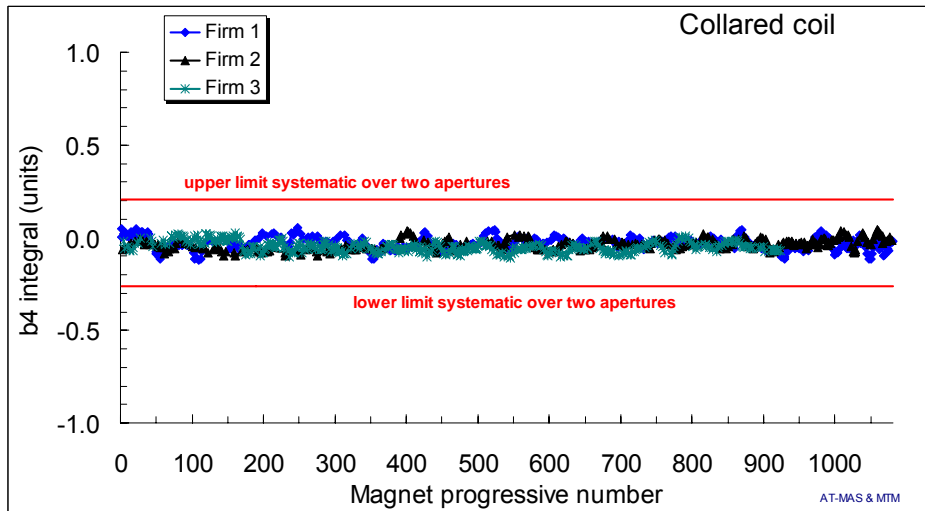
Fig. 22: Average b_4 in straight part of the collared coils (average of the apertures), separated per Firm (each dot is the average of 5 consecutive magnets of the same Firm), and beam dynamics targets for the systematic (red lines) based on correlations with 176 cryodipoles.
