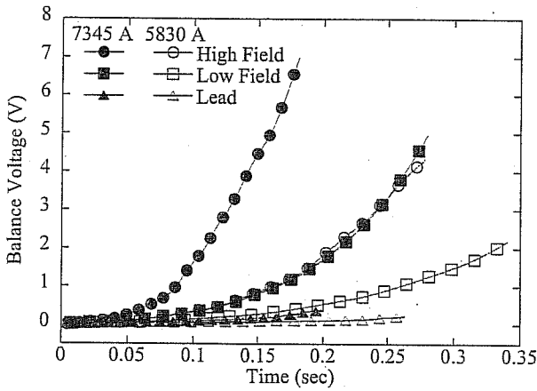
Fig. 5. Measured balance voltage rise at the heater quench tests at the current corresponding to 50 GeV and 40 GeV. t = 0 sec is the start time of the quench.
