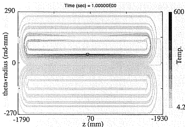
Fig. 7. The calculated temperature profile in 1.0 sec after the quench. The quench initiates at the center of the straight section at the high field side, pointed by an open circle.
