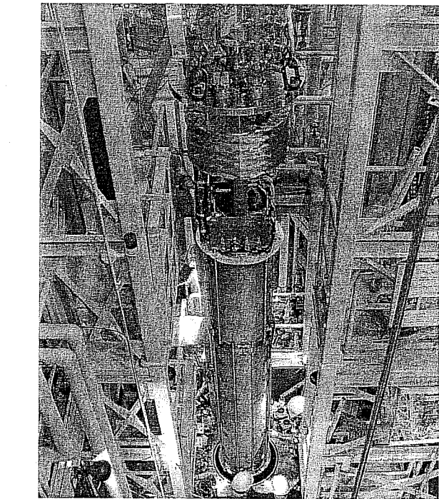
Fig. 2. Prototype magnet installation into the vertical cryostat.
