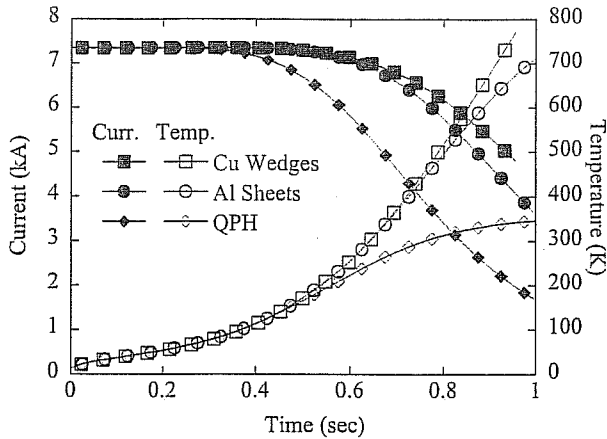
Fig. 10. The current and maximum temperature changes assuming the Al sheets, Cu wedges and quench protection heaters. The quench initiates at the lead on the median plane
