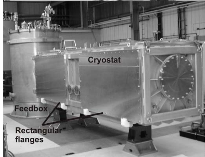
Fig. 2. Rectangular shaped all-purpose cryostat.
