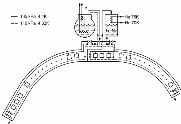
Fig. 2. The simplified scheme of cooling 1/3 part of the SIS100 ring.
