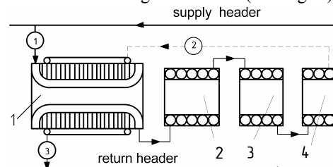
Fig. 1. The simplified flow diagram of the SIS100 module: 1 – a quadrupole lens; 2, 3 – a pickup, a multipole, a steerer or a collimator; 4 – additional tube for adjustment of hydraulic resistance of a module.
