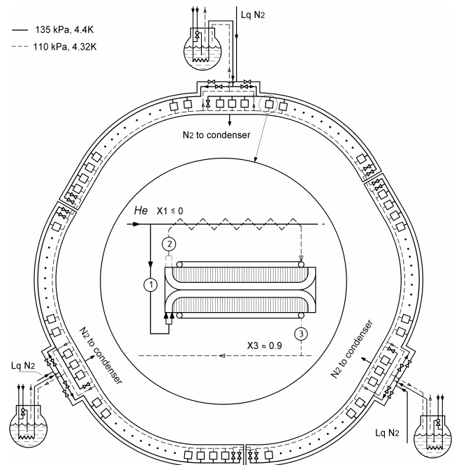
Fig. 3. The SIS300 ring cooling simplified flow diagram
